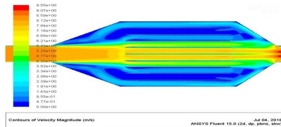
Fig 1.3: Velocity contour without diverter
