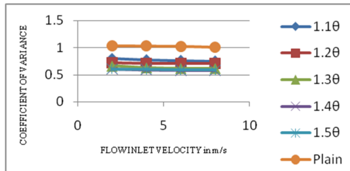
Graph 3.3: Effect of diverter length on Coefficient of variance for varying inlet velocity where l = 0.3L
