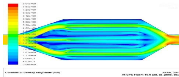
Fig 1.4: Velocity contour with diverter
