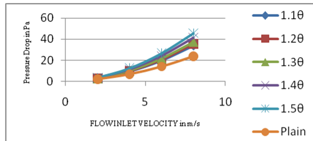
Graph 3.4: Effect of diverter length on pressure drop for varying inlet velocity where l = 0.5L
