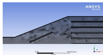
Fig 2.4: Unstructured mesh for 2D analysis of fluid flow with diverter
