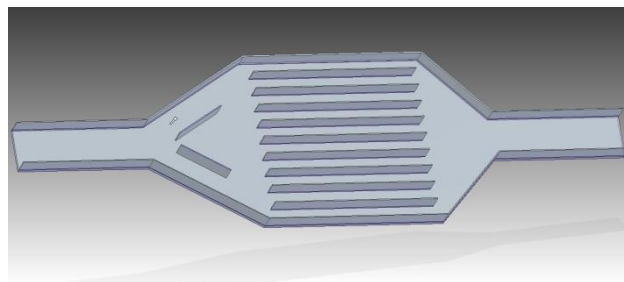
Fig 1.2: Heat sink with rectangular channels and diverter
