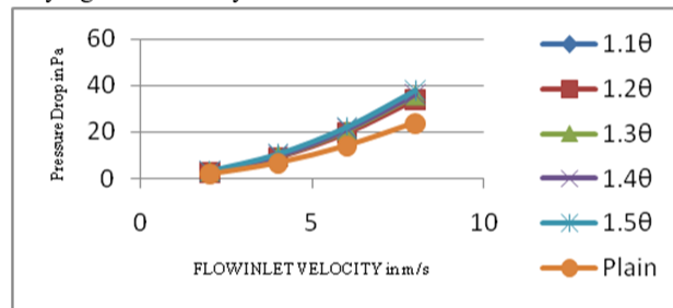
Graph 3.5: Effect of diverter length on pressure drop for varying inlet velocity where l = 0.4L
