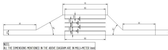
Fig 2.1: 2D Geometry of the Heat Sink Domain without Diverter
