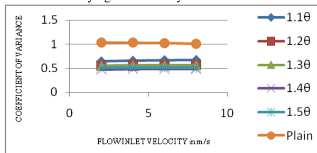
Graph 3.2: Effect of diverter length on Coefficient of variance for varying inlet velocity where l = 0.4L
