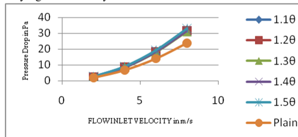
Graph 3.6: Effect of diverter length on pressure drop for varying inlet velocity where l = 0.3L
