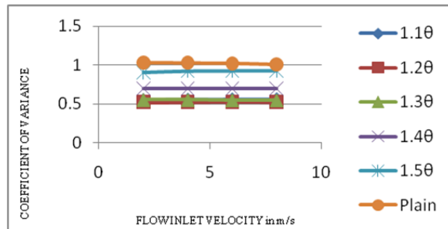
Graph 3.1: Effect of diverter length on Coefficient of variance for varying inlet velocity where l = 0.5L
